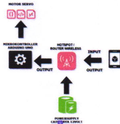
Gambar 1. Blok Diagram
